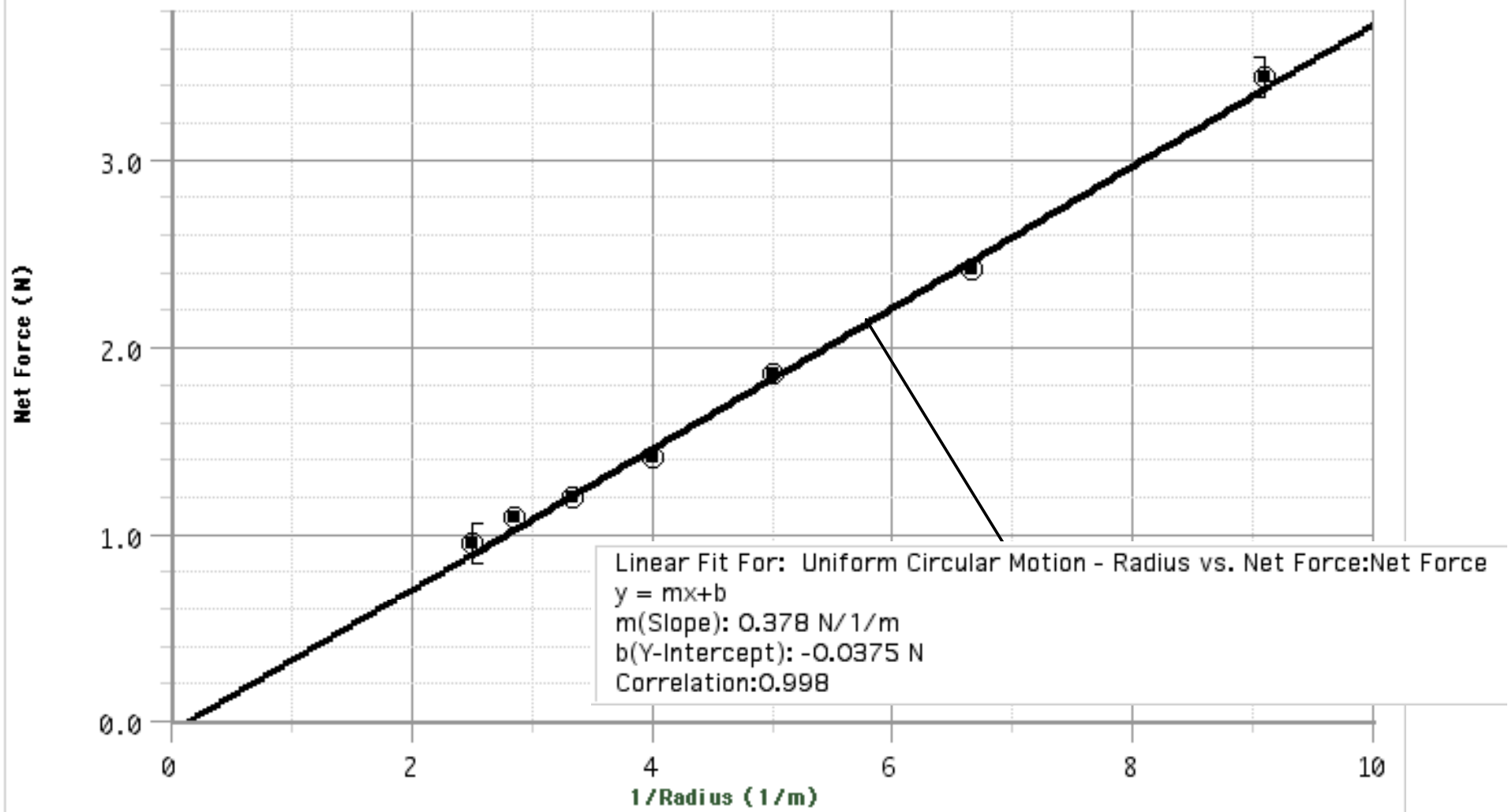
F vs. 1/radius - Uniform Circular Motion
