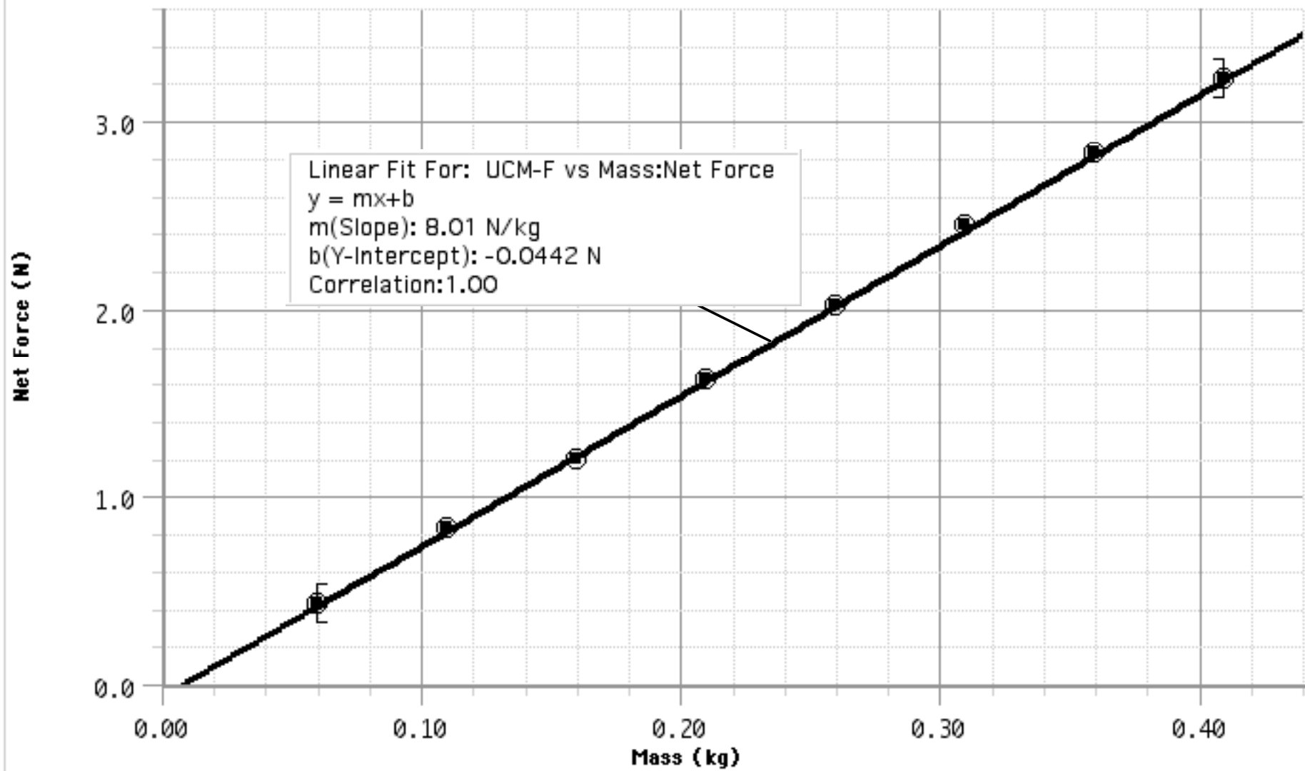
F vs. mass - Uniform Circular Motion
