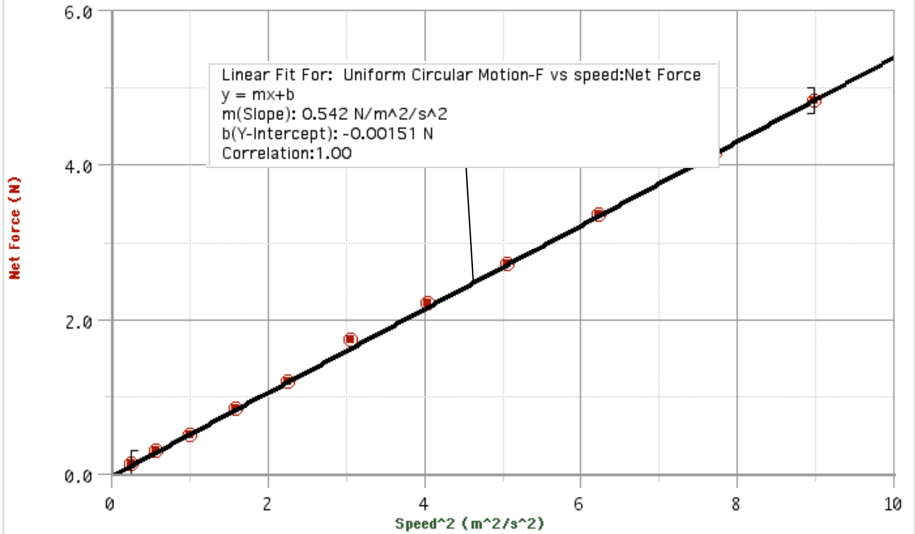
F vs. Speed 2 - Uniform Circular Motion
